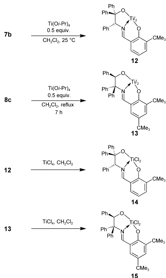
Scheme 5. Synthesis of bis-chelated titanium complexes 12 , 13 and generation of dichloro complexes 14 , 15 .
