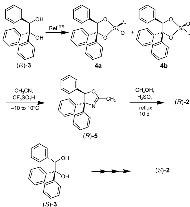
Scheme 2. Synthesis of ( R )- and ( S )-2-amino-1,2,2-triphenylethanol 2 .
