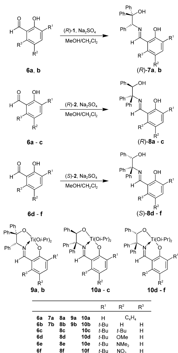
Scheme 3. Imines 7 , 8 and monochelated titanium complexes 9 , 10 derived from the regioisomeric amino alcohols 1 and 2 , respectively.
