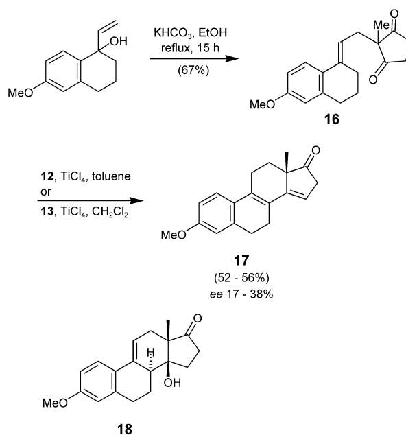
Scheme 6. Cyclization of meso -diene 16 to Torgov diene 17 , mediated by Lewis acids generated from titanium complexes 12 or 13 .
