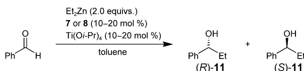
Scheme 4. Enantioselective addition of diethylzinc to benzaldehyde mediated by the imines 7 or 8 and titanium tetrakisopropoxide.
