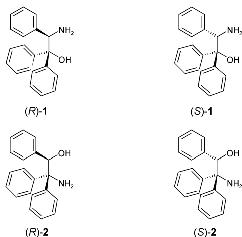
Scheme 1. The regioisomeric triphenylaminoethanols 1 and 2 .
